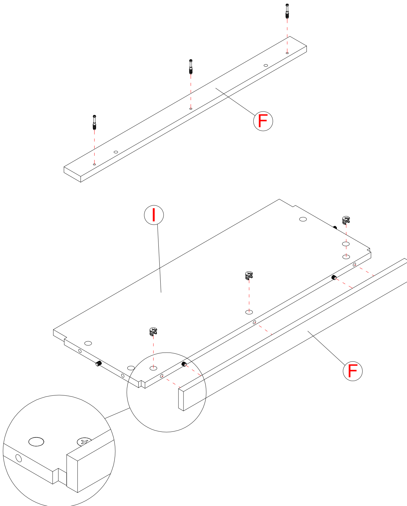
KD Cam
